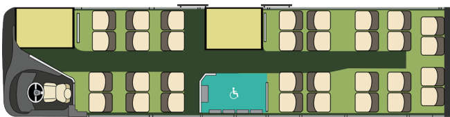
32+1 Seat layout two door
